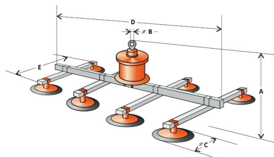
VMS 1200-8
