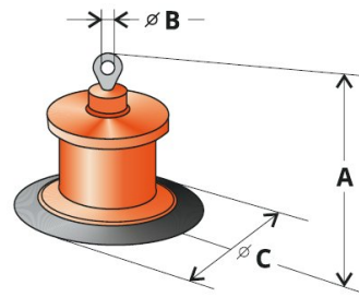
VMS 400 a VMS 1200-1
