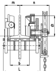
Z420-A(B) nosnost 1,6t; 3,2t; 5t; 7,5t a 10t
