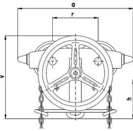
Z420-A(B) nosnost 1,6t; 3,2t; 5t; 7,5t a 10t
