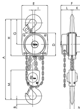
Yalelift 360 5.0t
