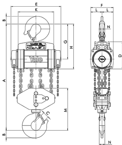
Yalelift 360 20.0t
