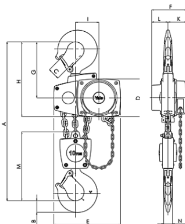
Yalelift 360 10.0t
