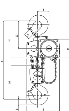
Yalelift 360 10.0t
