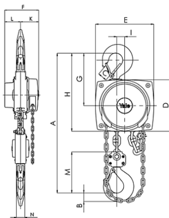
Yalelift 360 0.5t - 3.0t
