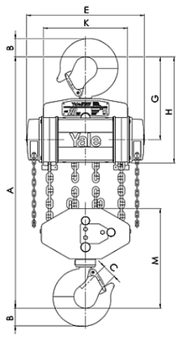
Yalelift 360 20.0t
