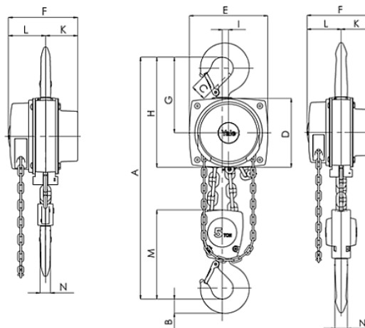
Yalelift 360 5.0t
